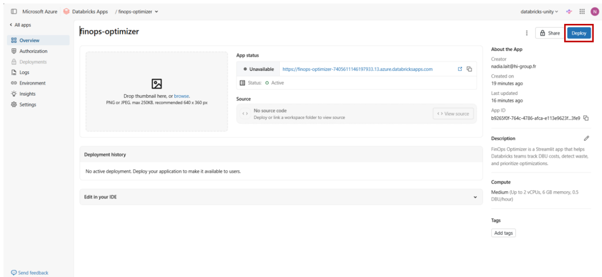
FIGURE 9 – Bouton Deploy .
